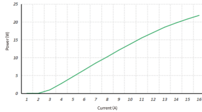
1470-10W Power curve
