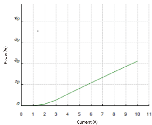
1060-10W Power curve
