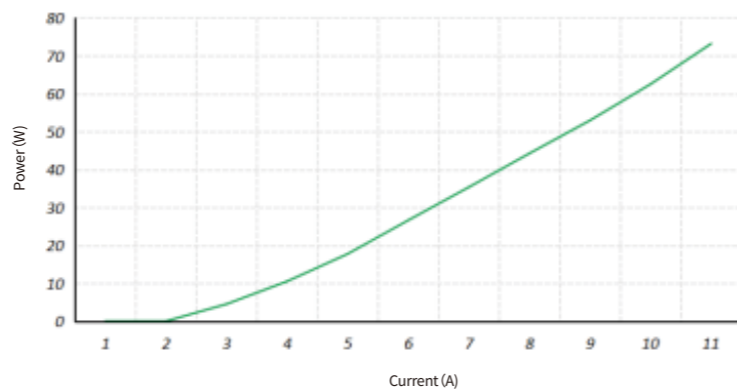
1060-70W Power curve
